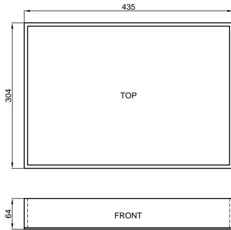
DRAWING #1 UPPER TRAY PLYWOOD CONSTRUCTION
