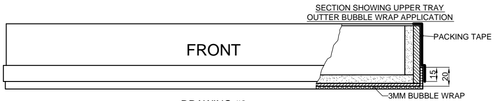
DRAWING #3 TRAY BOTTOM LINING
